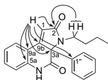
Figure 1. Selected HMBC correlations for 3f .
